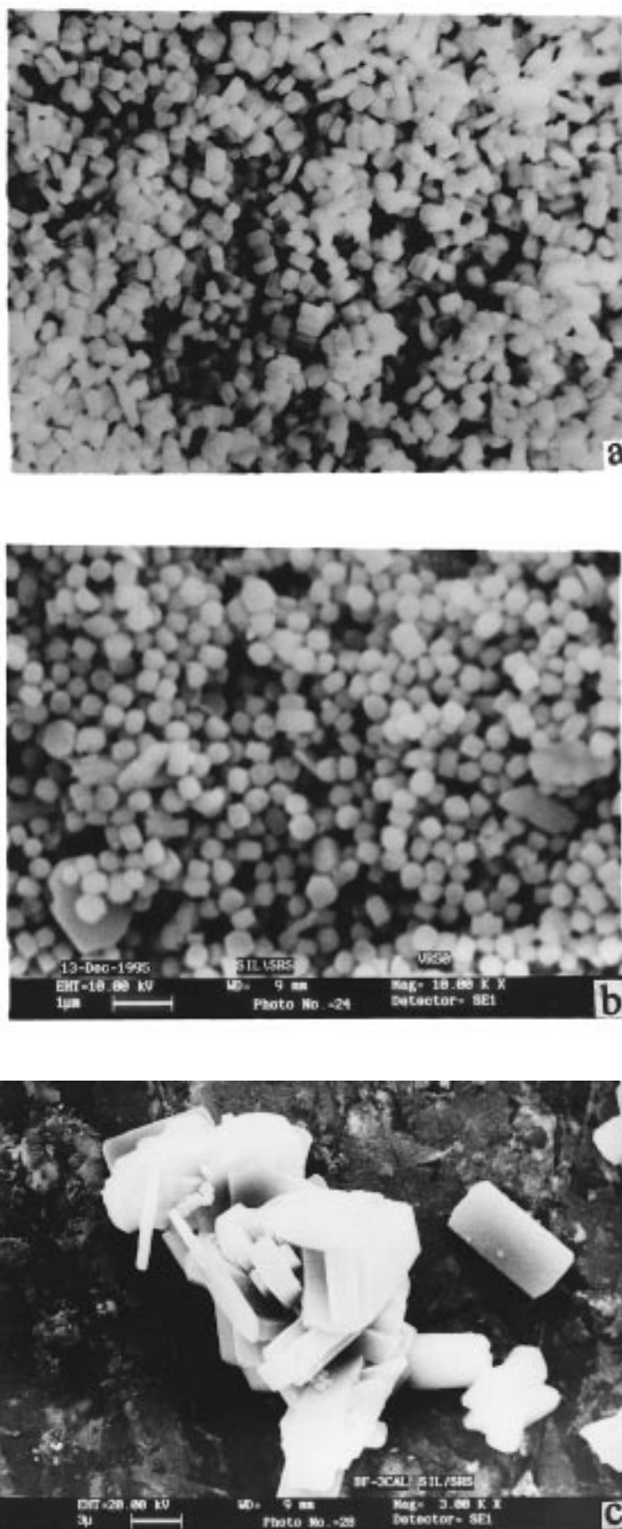
Figure 2. Scanning electron micrographs of Zr-Sil-1 sample A (a), sample D (b), sample F (c) and Sil-1 (d). (Continued on next page.)
