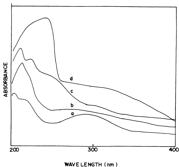
Figure 5. DR UV-Visible spectra of Zr-impregnated Sil-2 (a), Zr-Sil-1 sample C (b), sample E (c) and pure \text{ZrO}_2 (d).
